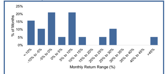
RM Bitcoin Monthly Performance Distribution
