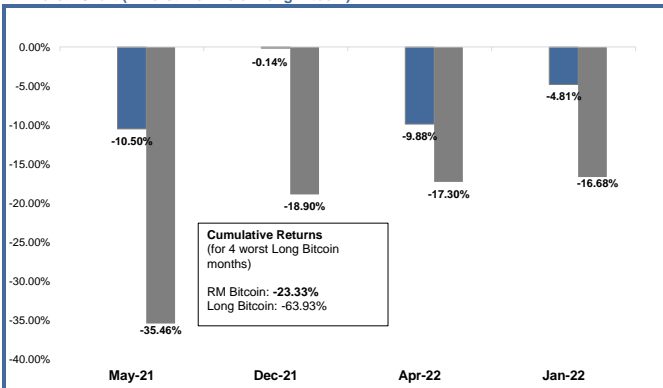
"4 Worst" Chart (4 worst months of Long Bitcoin)
